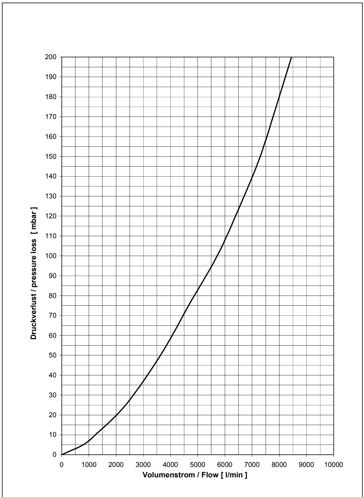
Fig. 1 Pressure loss Medium: Air at p_0 = 1013 \text{ mbar} , T_0 = 273\text{K} , density = 1,293 \text{ kg/m}^3
