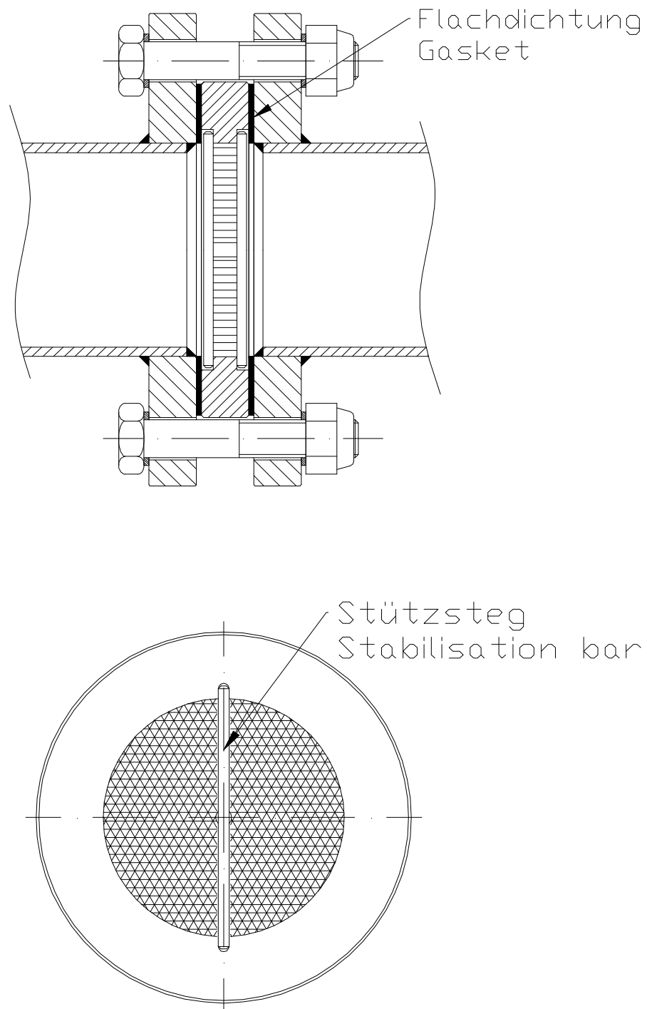
Fig. 1 Construction and assembly
